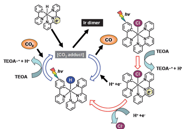
Scheme 1. Proposed mechanism for photocatalytic CO 2 reduction with [Ir-ppy] in MeCN/TEOA solution. TEOA = triethanolamine.
