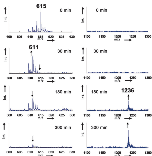
Figure 3. Steady-state measurements of changes in the ESI-MS spectra of a CO 2 -saturated MeCN/TEOA (5:1) solution containing [Ir-ppy] during irradiation at wavelengths in the range of 410 \leq \lambda \leq 750 nm.
